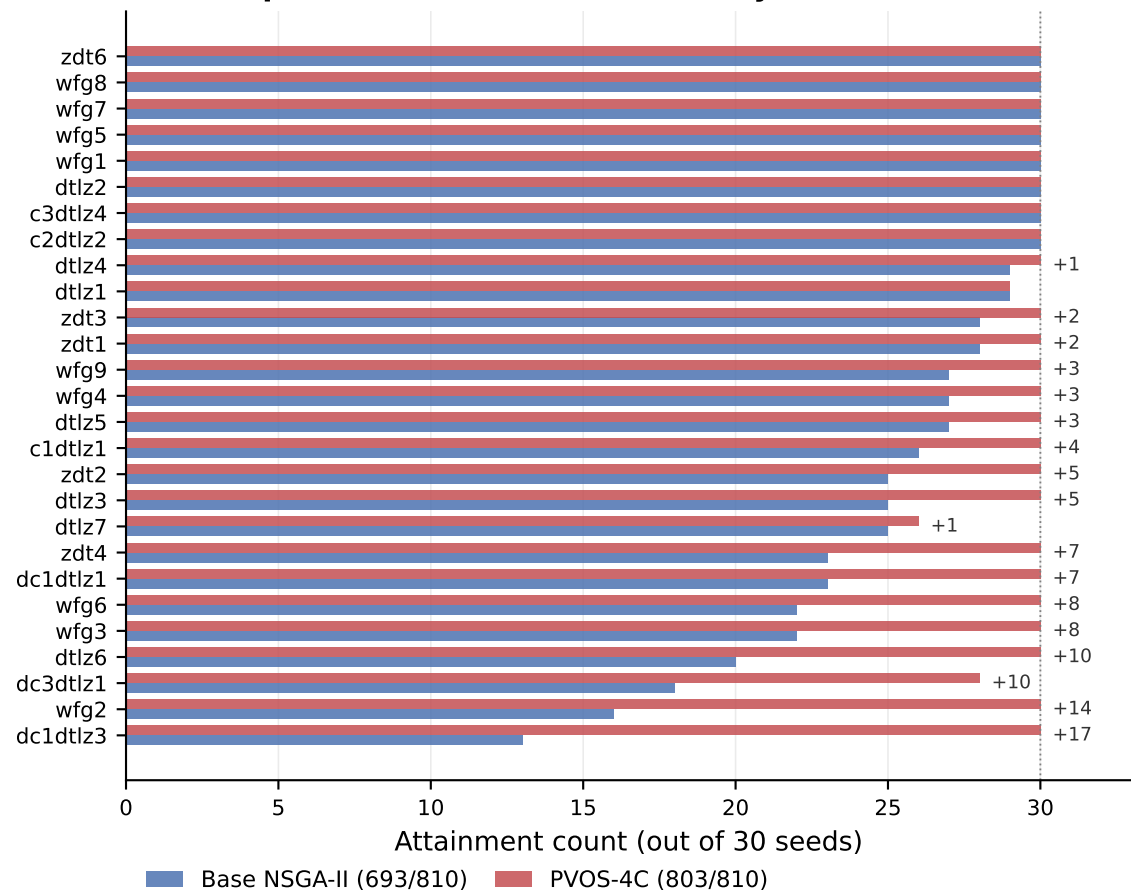
(b) Per-problem attainment, sorted by Base NSGA-II ascending
