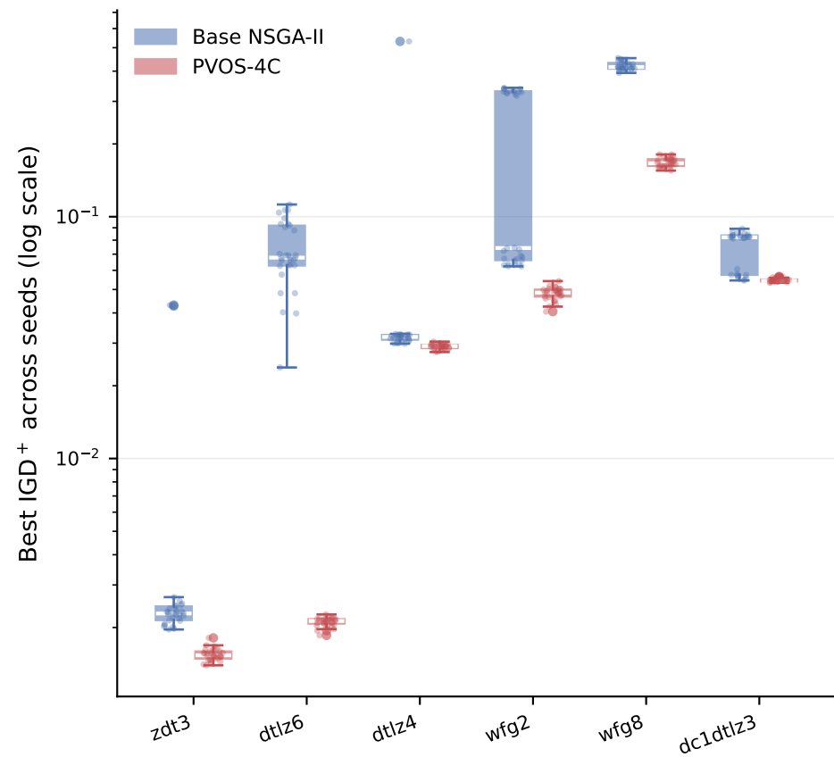
(a) Distribution of run-best IGD +
